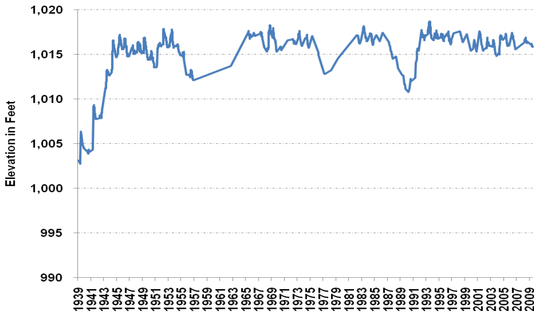
Figure 5. Madison Lake water levels history
