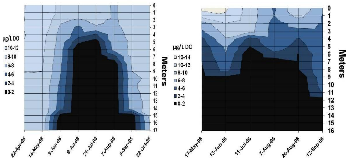
Figure 21. 2006 and 2008 interpolated dissolved oxygen isopleths
