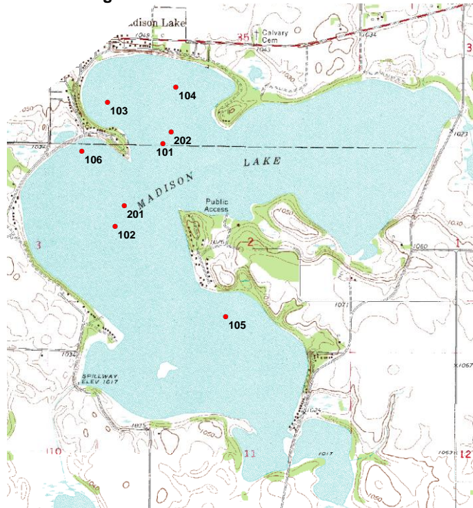
Figure 16. Madison Secchi transparency comparison among sites
